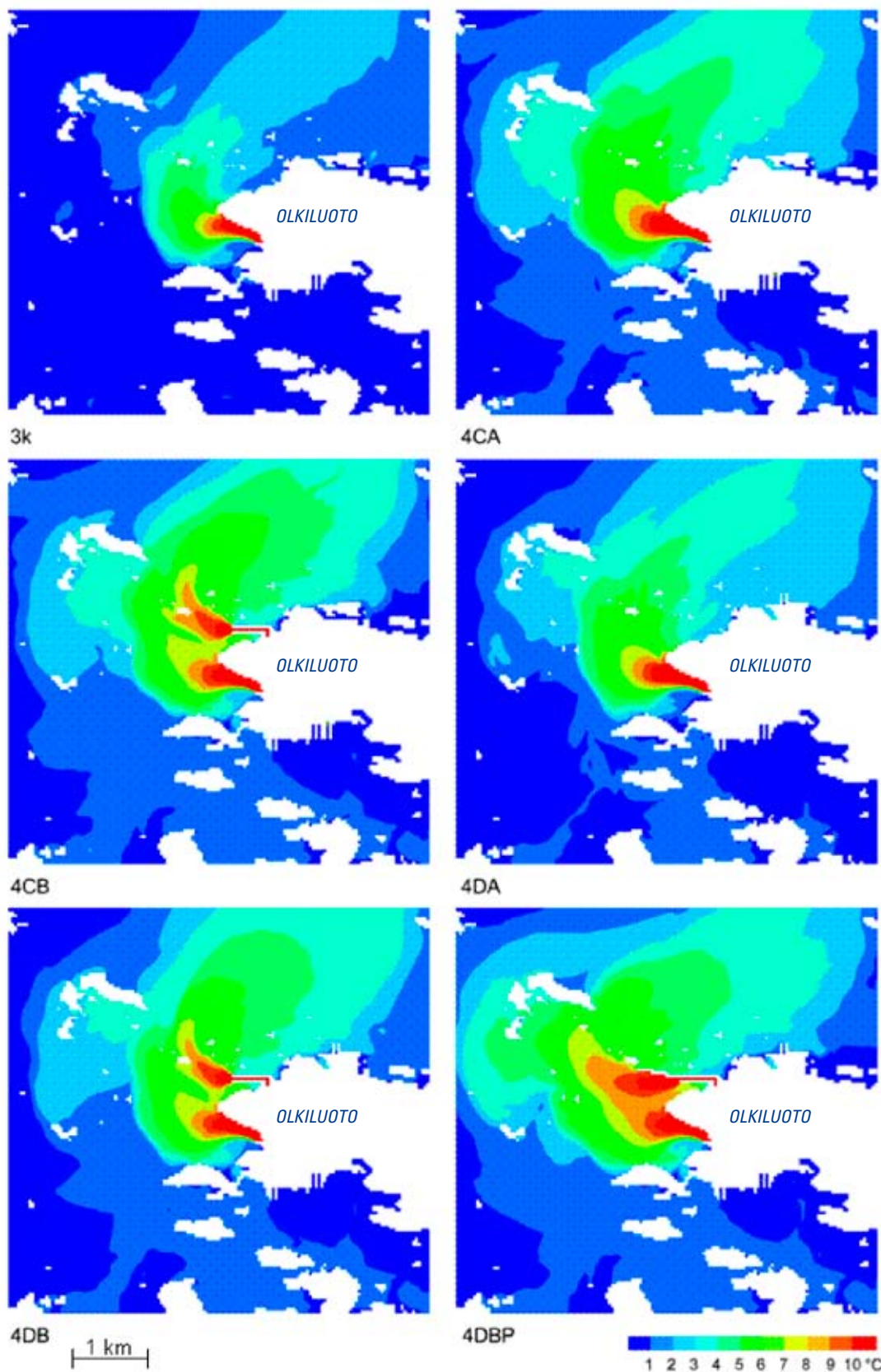
Figure 9-38 The increase in temperature caused by cooling water in the surface layer in a summertime example situation with wind coming from the south, calculated using the model. Alternatives explained in the text.
