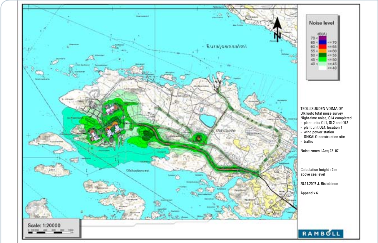
Figure 9-17 OL4 location option 1, night-time noise.
