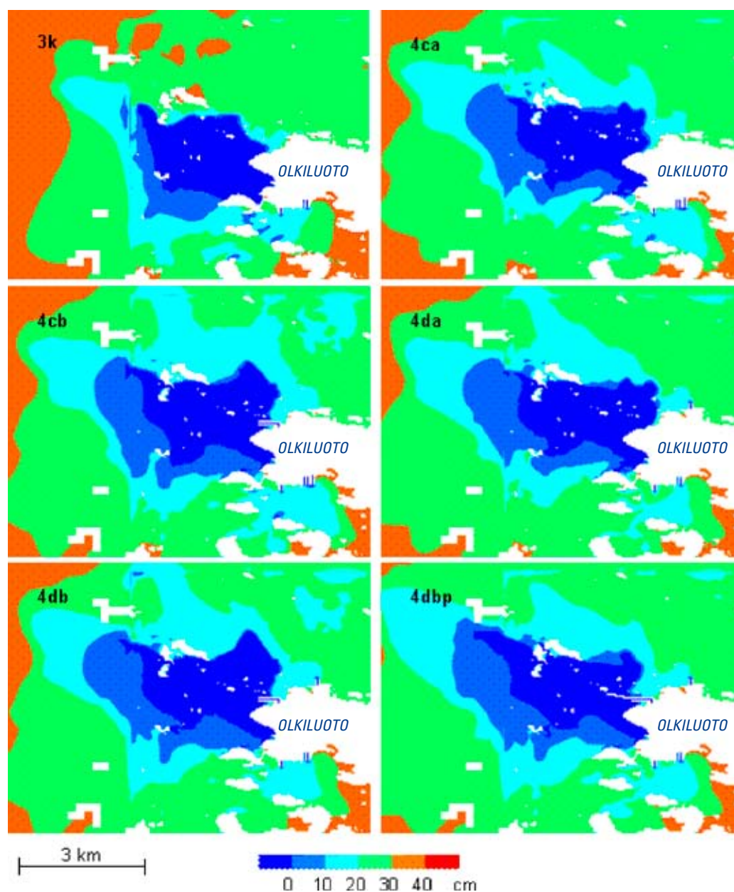
Figure 9-43 Ice conditions and ice thickness in the situation corresponding to the zero option (3k) and the impact of the new unit with different alternatives of intake and discharge locations.
