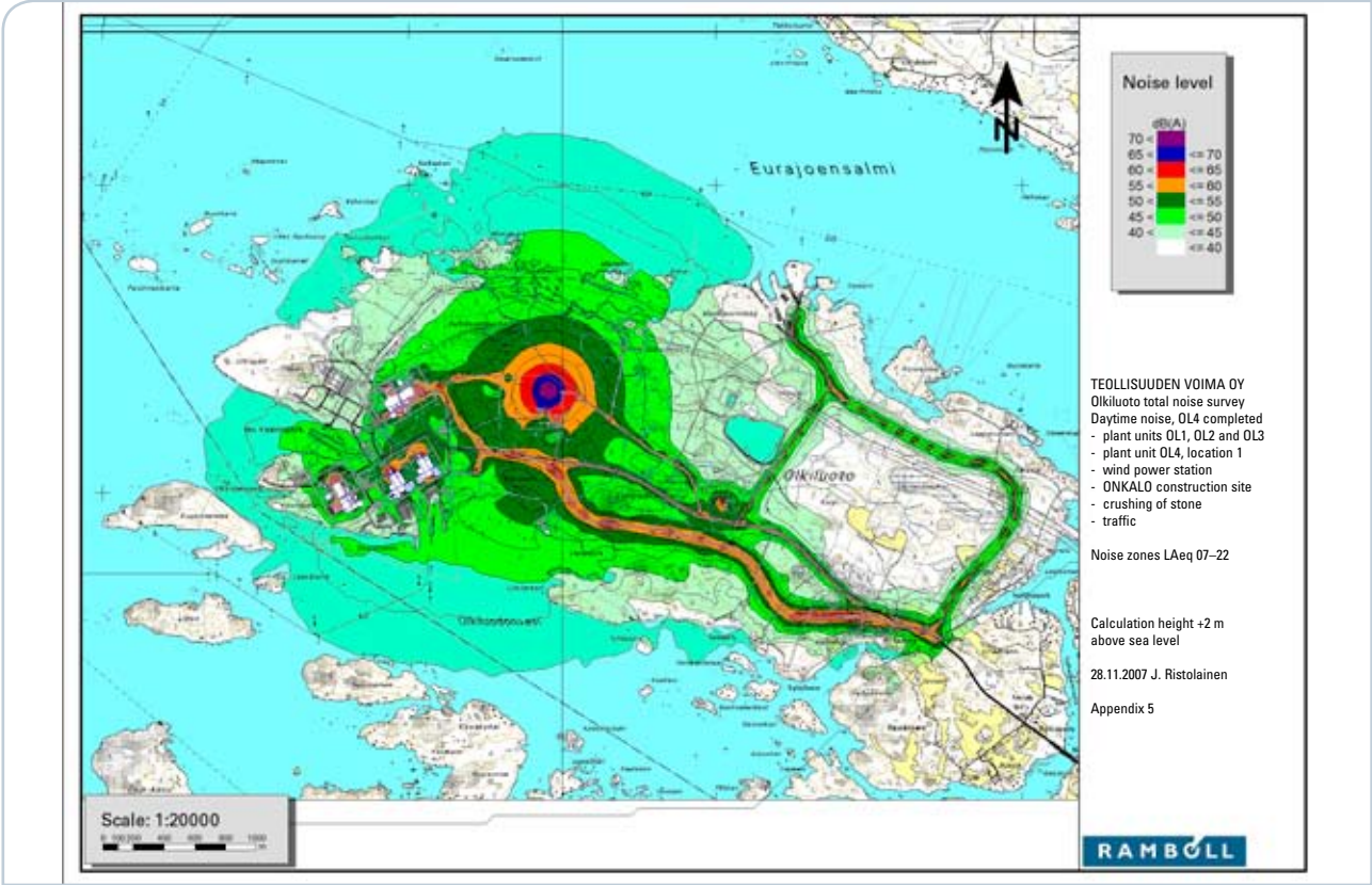
Figure 9-16 OL4 location option 1, daytime noise.
