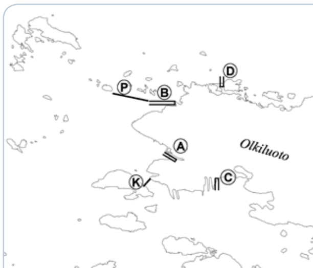
Figure 9-37 Cooling water intake and discharge points.
