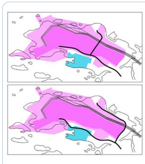
Figure 2-6 The present road network of Olkiluoto and the solution presented in the partial master plan proposal. A new road connection will be routed from the south side of the energy supply area directly to the present gate of the power plant site, while another road continues to the harbour along the eastern and northern borders of the energy supply area.
