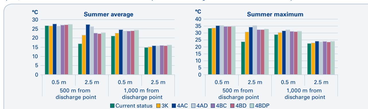
Figure 9-41 Calculated temperatures off the existing cooling water discharge points in the present situation, with the OL3 unit in operation (zero option) and with the different alternatives of the OL4 unit in operation as an average over the summer. Alternatives explained in the text.
