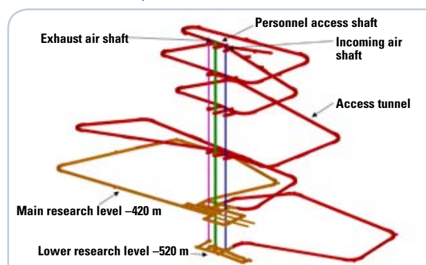
Figure 9-4 Structure of ONKALO. ONKALO is an underground rock characterisation facility (Posiva).
