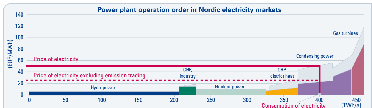
Figure 11-2 Determination of electricity price in the Nordic electricity market. The area shaded in grey represents the increase in electricity production costs at an emissions right price of €20/tCO 2 .
